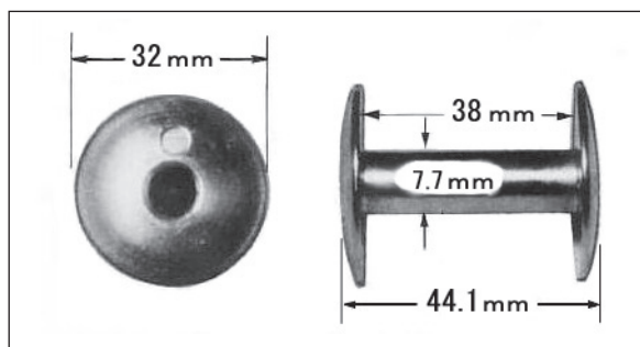
Large bobbin
