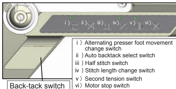
Back-tack switch
