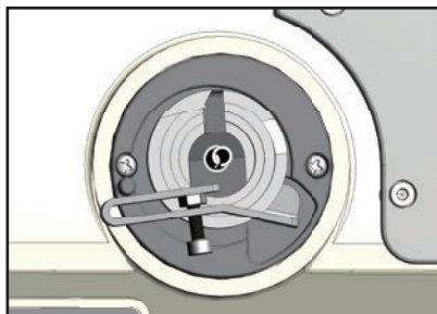
Built-in bobbin winder with winding amount fine adjuster
