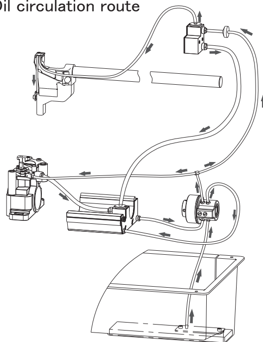
油の循環経路／ Oil circulation route
